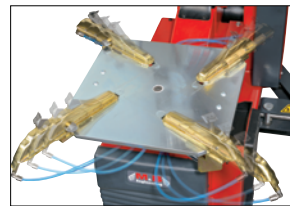
Turntable with mobile clamps (TC-328it)
